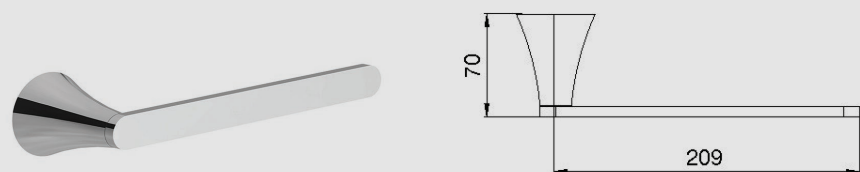
FV163/K4 Toallero corto. PC-BB-BG-BK-BN PB-BHB-UPB-PN-SGR
