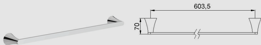
FV164.01/K4 Barral 600 mm. PC-BB-BG-BK-BN PB-BHB-UPB-PN-SGR
